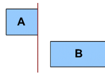
Figure 8. Non-concurrent tasks
